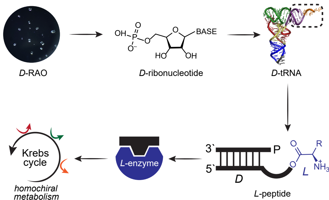
FIG. 3. Propagation of homochirality from a common ribonucleotide precursor, RAO, to the entire prebiotic network is illustrated. D-RAO can be transformed into D-ribonucleotides, forming homochiral RNA. L-peptides can be synthesized through the stereoselective binding of L-amino acids to tRNA analogs composed of D-ribonucleotides. This crucial link enables the transfer of homochirality from nucleic acids to peptides. Then L-peptides form L-enzymes, and by enantioselective catalysis a homochiral metabolism can be produced.
