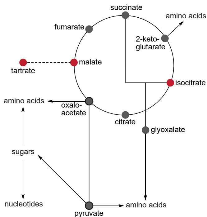
FIG. 2. Core metabolism—absent catalysis by enzymes, cannot propagate chiral information. The two chiral entities (L-malate and D-isocitrate, shown in red) are flanked by achiral intermediates (shown in gray). Making matters worse, the achiral branch points (oxaloacetate and pyruvate) inhibit the flow of chiral information from/through the metabolites. The theoretical provisioning of metabolism using chiral tartrate as a precursor is indicated by the dashed line.
