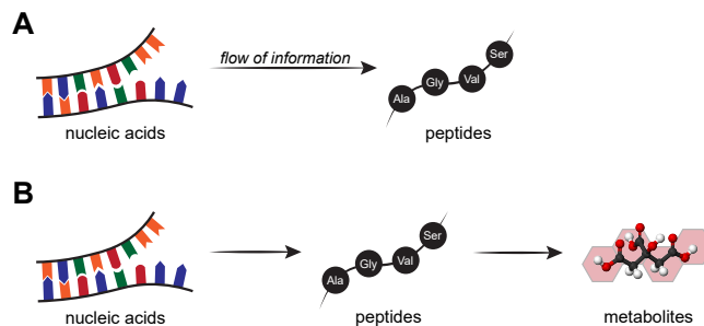
FIG. 1. A) The central dogma of molecular biology, as established by Francis Crick, states that once the information has passed into proteins, it cannot get out. Therefore, the flow of genetic information is unidirectional, from nucleic acids to peptides. B) The central dogma can be expanded to include another molecular class: metabolites, because a metabolic network comprises compositional information determined by nucleic acids and peptides.
