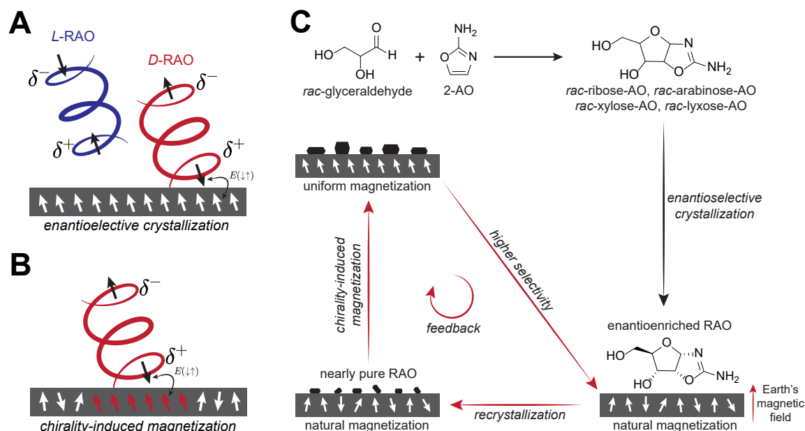
FIG. 4. A ) Due to the CISS effect, magnetic surfaces with net magnetization can function as chiral agents and be templates for the enantioselective crystallization of RAO from its racemic solution, by a spin-controlled process. B ) Selective interaction of chiral molecules with the electron spin can be utilized to magnetize magnetic surfaces. Magnetic surfaces with no net magnetization can be uniformly magnetized by crystallization of enantiopure RAO, along the chiral molecular axis. C ) Enantioselective crystallization of chiral molecules on magnetic surfaces can be considered together with the chirality-induced magnetization in a cooperative feedback. With this feedback, a small bias in the natural magnetization of magnetic surfaces due to the geomagnetic field can be amplified, and enantioselective processes controlled by the electron spin can be made highly efficient. Note that racemic RAO is synthesized with three other racemic aminooxazolines (arabinose-AO, xylose-AO, lyxose-AO), which get excluded in the initial crystallization step due to the relatively low solubility of RAO.
